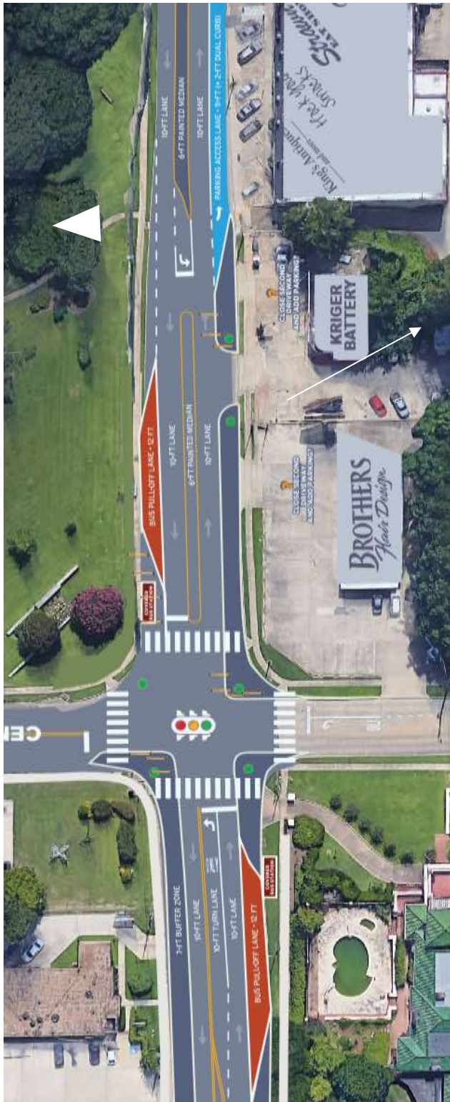
Figure 7.8 – Kings Highway Congestion Mitigation Project: Road/Traffic Diet and Additional Geometric/Safety Features
